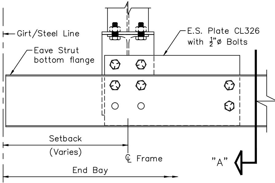
Eave Strut Connection Detail
